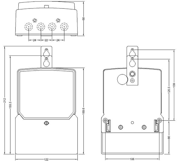
METER DIMENSIONS – LONG COVER
