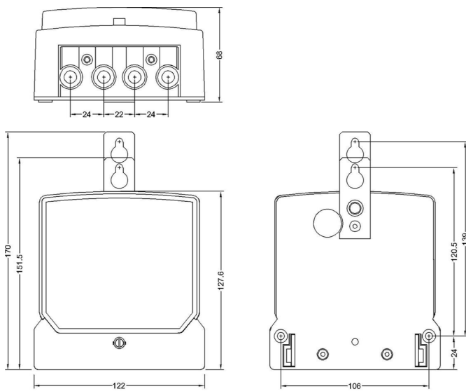
METER DIMENSIONS - SHORT COVER
